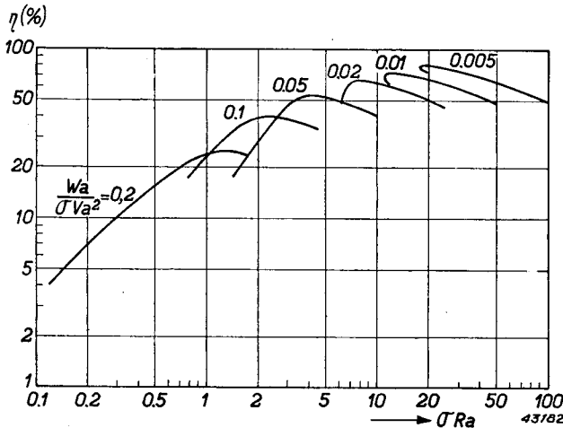
Fig. 34. \eta as function of \sigma R_a , with W_a/\sigma V_a^2 as parameter.
