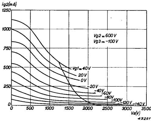
Fig. 87. As fig. 86, but at V_{g3} = -100 V.
