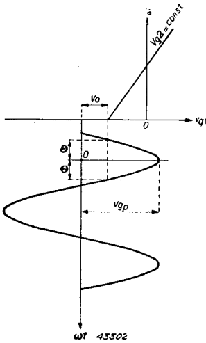
Fig. 137. Ideal i_a-v_{g1} characteristics for class C excitation.
