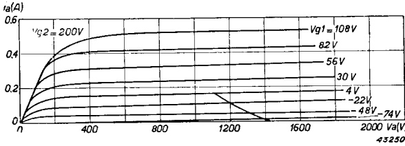
Fig. 76. As Fig. 73, but with V_{g2} = 200 V.
