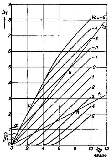
Fig. 138. Excitation characteristics giving I_{a1} = f(V_{gp}) , with V_o as parameter, under the conditions obtaining in fig. 137.
