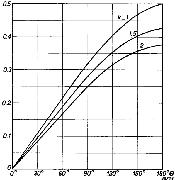
Fig. 18. The relation I_{ao}/I_{ap} = f_o(\theta) as function of the half current angle \theta in respect of an i_a/v_s characteristic of the type i_a = cv_s^k , at k = 1-1.5 and 2.
