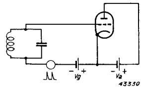
Fig. 175. Circuit in which instability will occur due to secondary grid emission.
