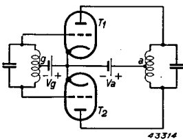
Fig. 151. Balanced oscillator with feedback across the anode-grid capacity.
