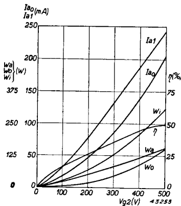
Fig. 79. Screen grid modulation characteristic of a pentode, based on the dates from figs. 73 to 77.
